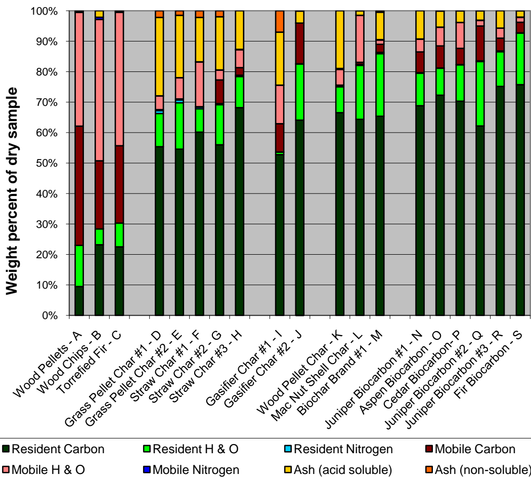
FIGURE 6: MODIFIED ULTIMATE ANALYSES OF CHARs
