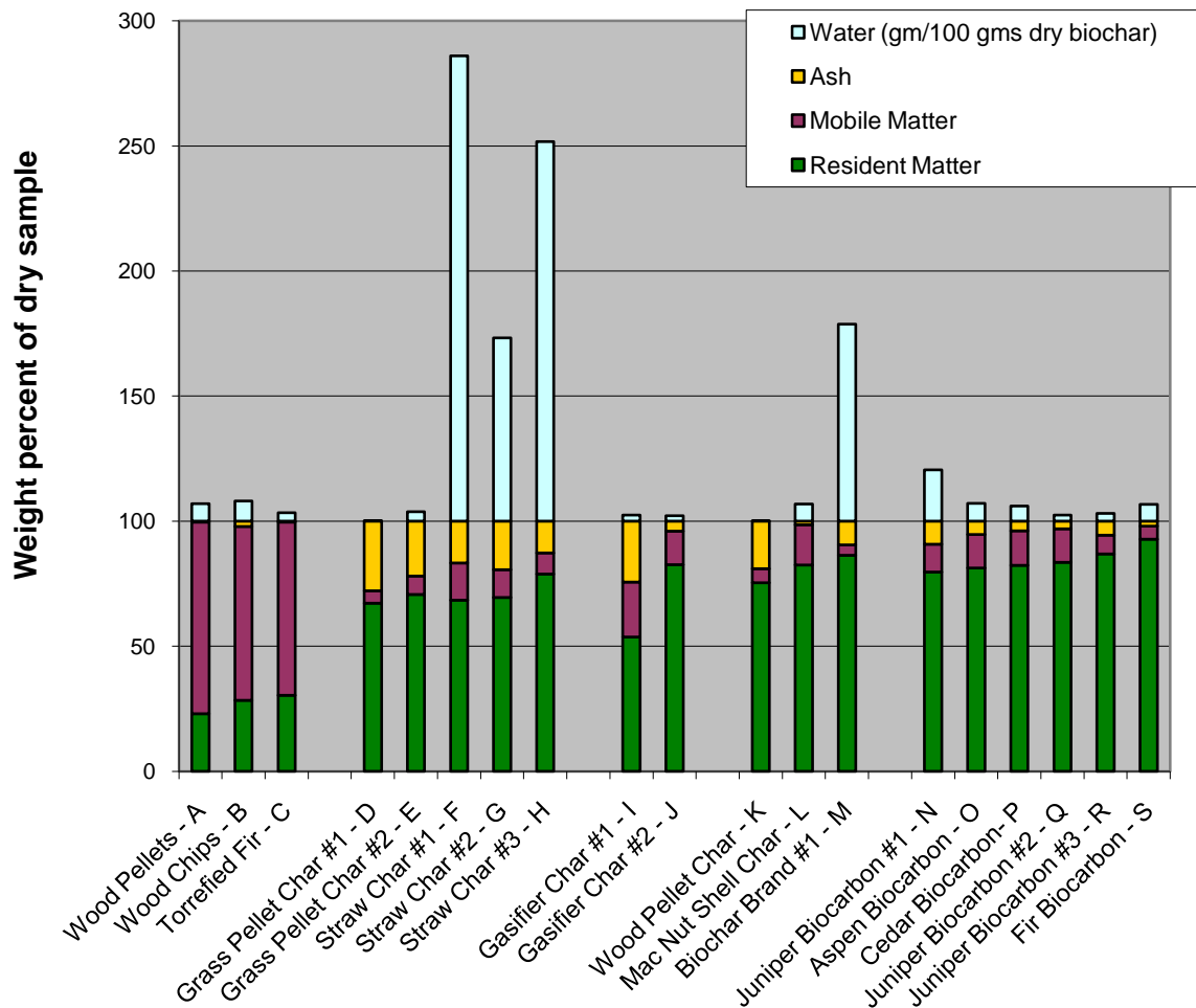
FIGURE 5: MODIFIED PROXIMATE ANALYSES OF CHARS
