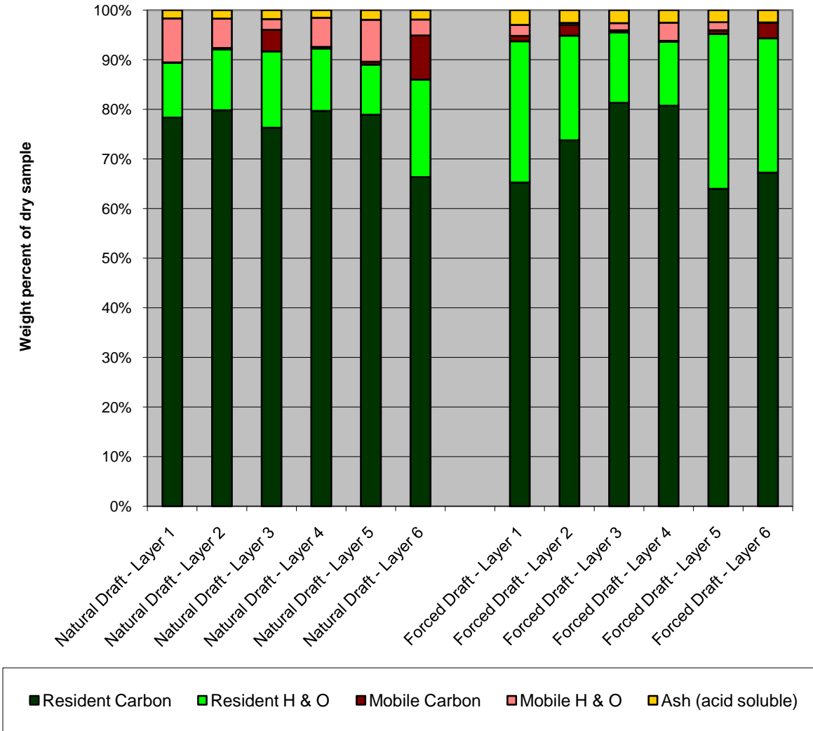
FIGURE 15: MODIFIED ULTIMATE ANALYSES OF TLUD CHARS
