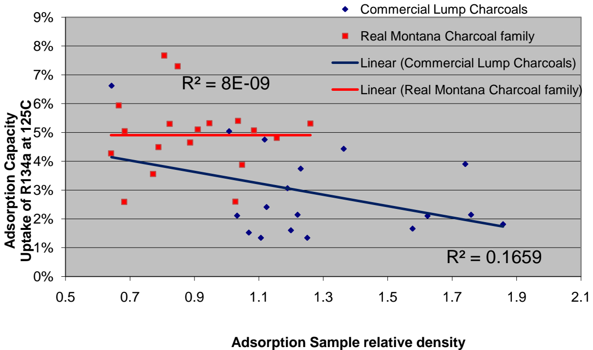
FIGURE 11: REAL MONTANA CHARCOAL ADSORPTION CAPACITIES
