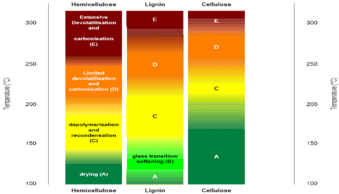
FIGURE 2: THERMAL MODIFICATIONS OF WOOD CONSTITUENTS
