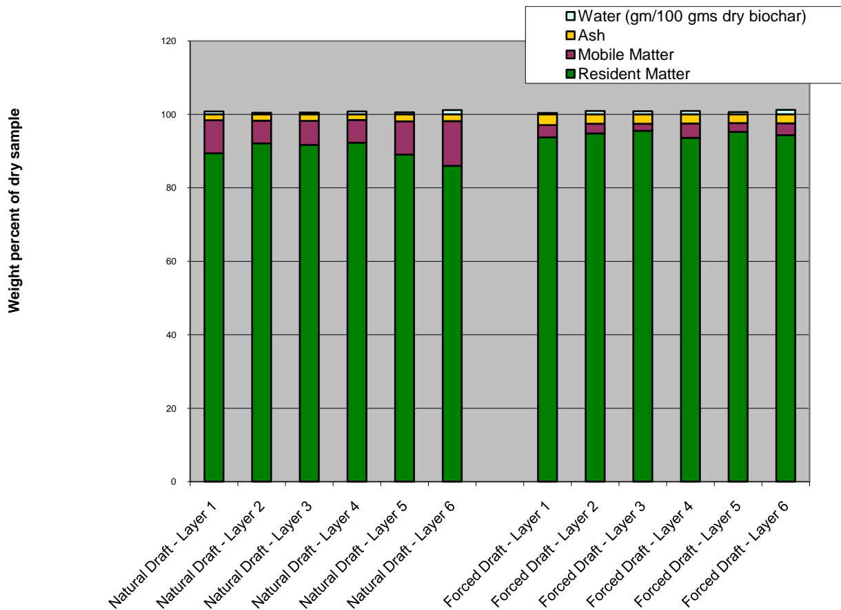
FIGURE 14: MODIFIED PROXIMATE ANALYSES OF TLUD CHARS
