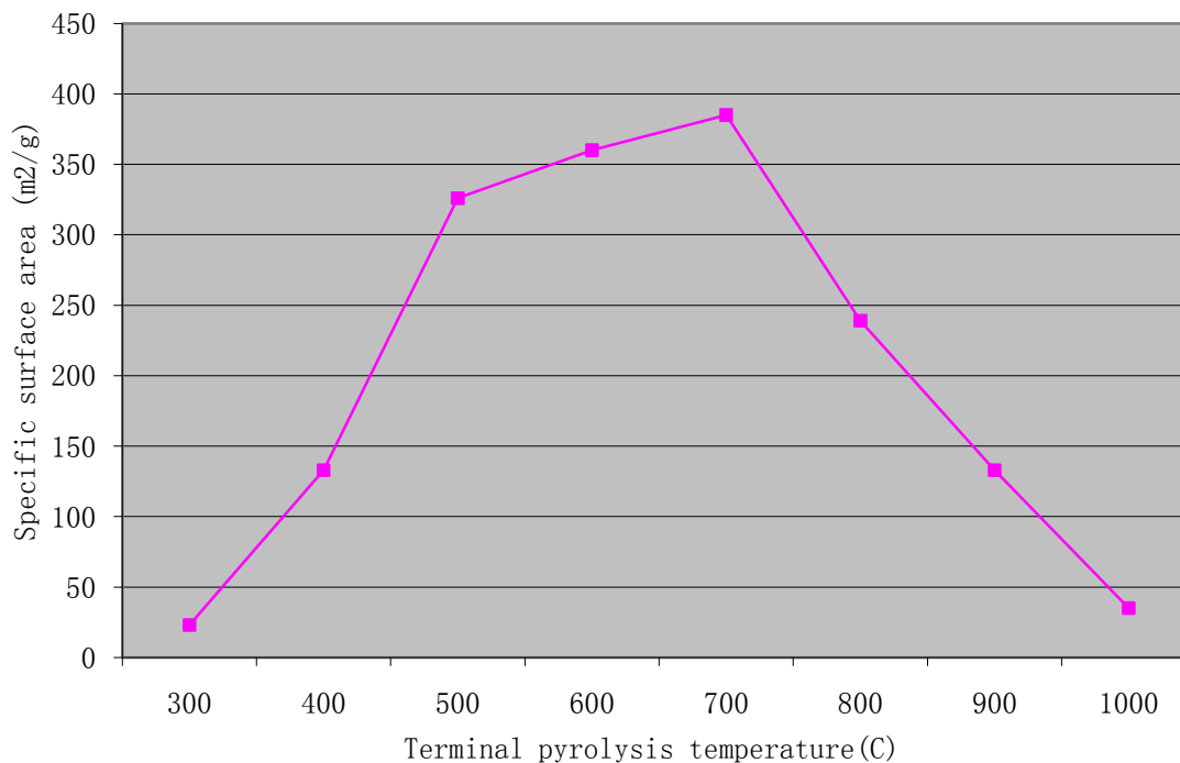
FIGURE 7: VARIATION OF CHAR BET SURFACE AREA WITH HTT
