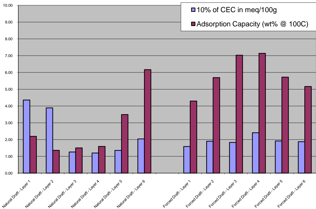
FIGURE 16: CEC AND ADSORPTION CAPACITY OF TLUD CHARS
